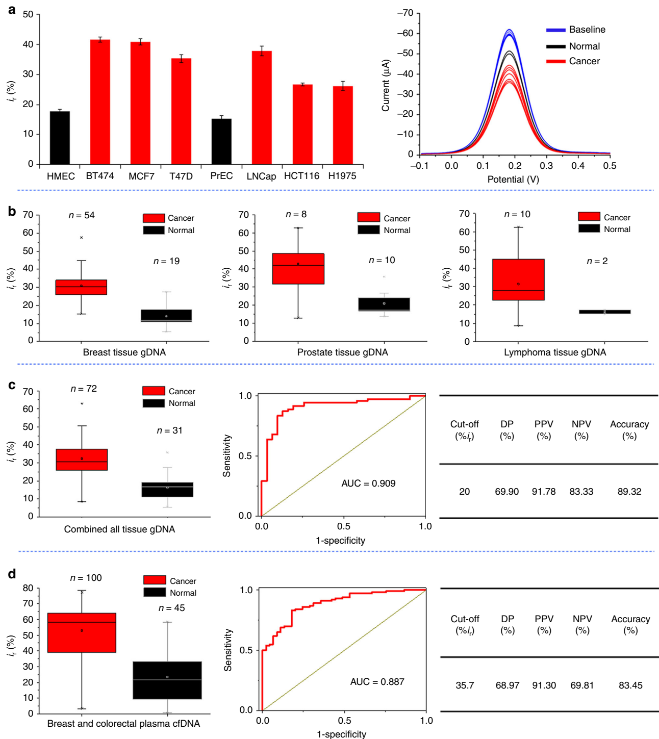
Fig. 3 Practical application of Methylscape approach. a Differential affinity/adsorption of genomic DNAs as a function of their cancer and normal origin. Bars represent the relative current ( I_r ) mean values for DNA genomes derived from various normal (Black bars: Human Mammalian Epithelial Cell (HMEC), Prostate Epithelial cell (PrEC)) and cancer cell lines (Red bars: Breast cancer: BT474, MCF7, T47D, LNCap prostate cancer, HCT116 colorectal cancer and H-1975 lung cancer). Each data point represents the average of three separate trials, and error bars represent the standard deviation of measurements ( \%RSD < 5\% for n = 3 ). Right panel: Corresponding DPV graphs for all cell line DNAs and their respective baseline. b Individual box plot showing mean relative current ( I_r ) values generated by electrochemical detection of genomic DNAs extracted from normal and cancer tissues of various cancer types (breast, prostate and lymph node). c The combined data for all the tissue samples derived from 31 healthy individuals and 72 cancer patients, Right: the ROC analysis and diagnostic test evaluation shows the Disease Prevalence (DP), positive predictive values (PPV), negative predictive values (NPV) and accuracy of the method. d Box plot showing relative current ( I_r ) mean values generated by electrochemical detection for genomic DNAs extracted from plasma samples derived from 45 healthy individuals and 100 breast cancer patients, Right: the ROC analysis and diagnostic test evaluation shows the Disease Prevalence (DP), positive predictive values (PPV), negative predictive values (NPV) and accuracy of the method. In the box and whisker plots, the middle lines of the boxes represent the median (50th percentile) and the terminal line of the boxes represents the 25th to 75th percentile. The whiskers represent the lowest and the highest value
